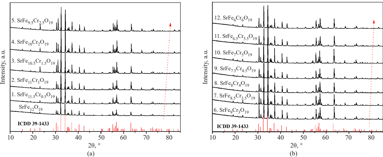
Fig. 1. XRD patterns of SrFe 12-x Cr x O 19 system: (a) x = 0–2.5; (b) x = 3–6
